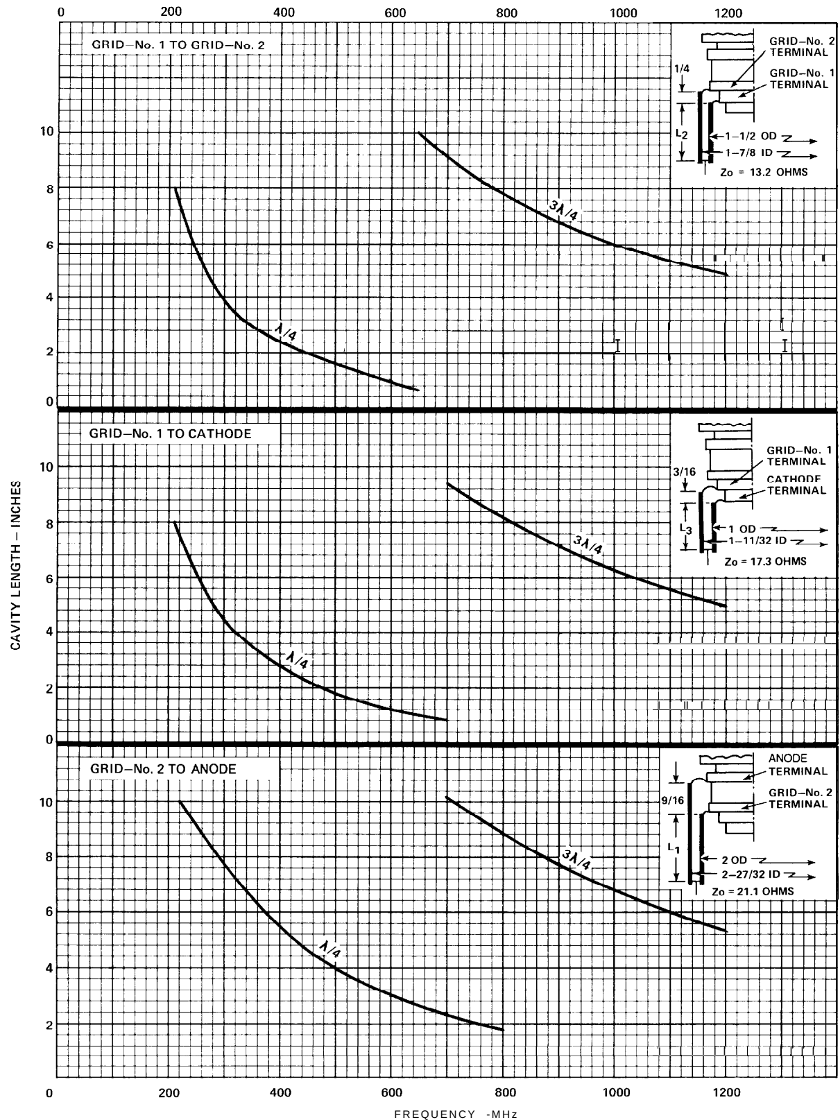
Figure 2 • Tuning Characteristics
