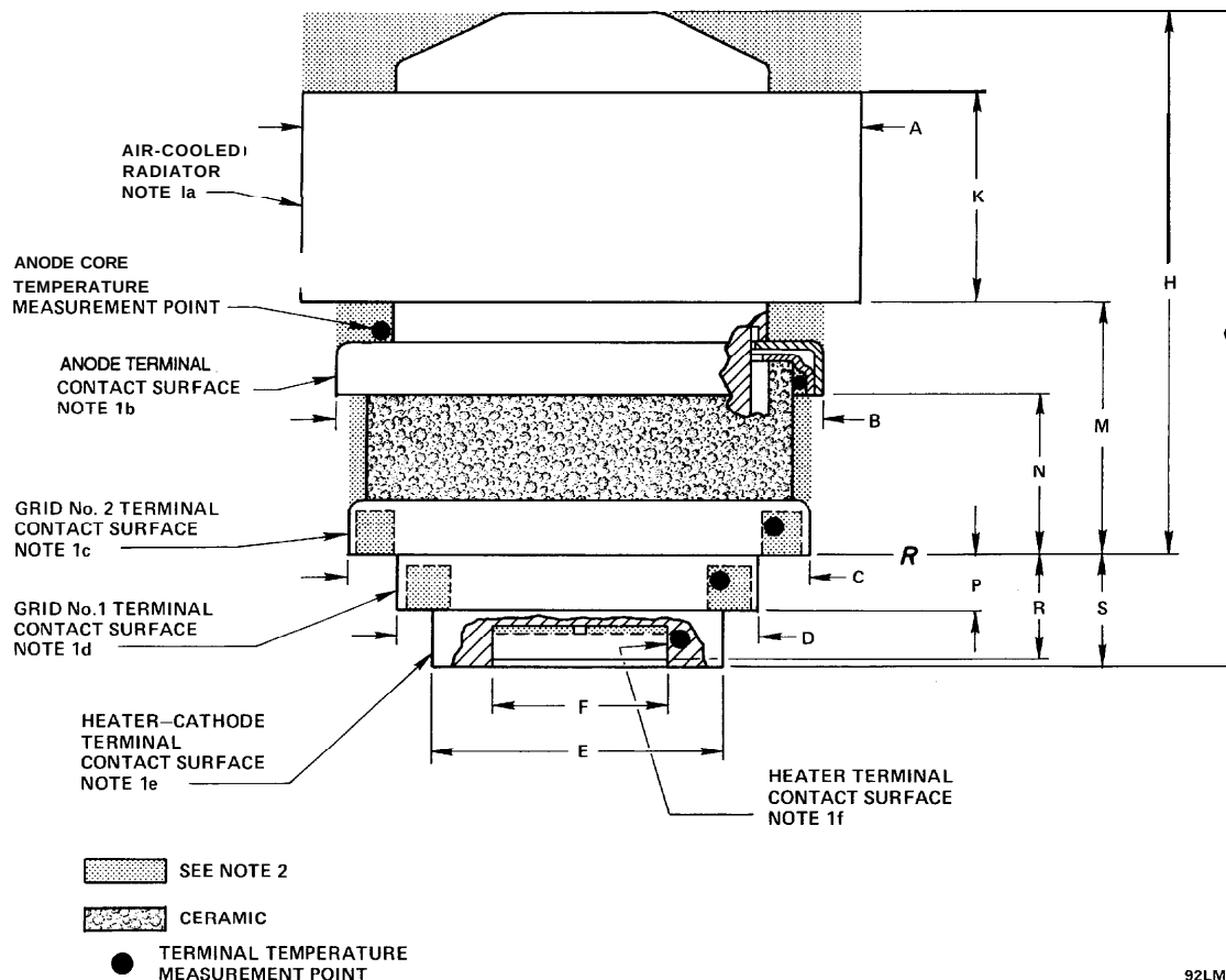
Figure 5 - Dimensional Outline
