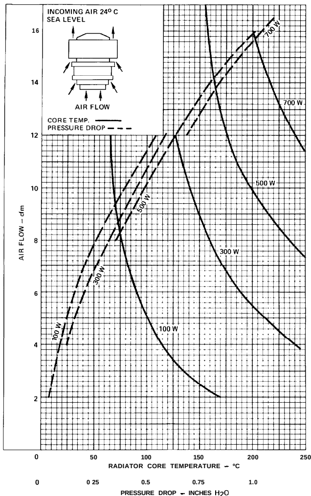
Figure 6 - Cooling Characteristics
